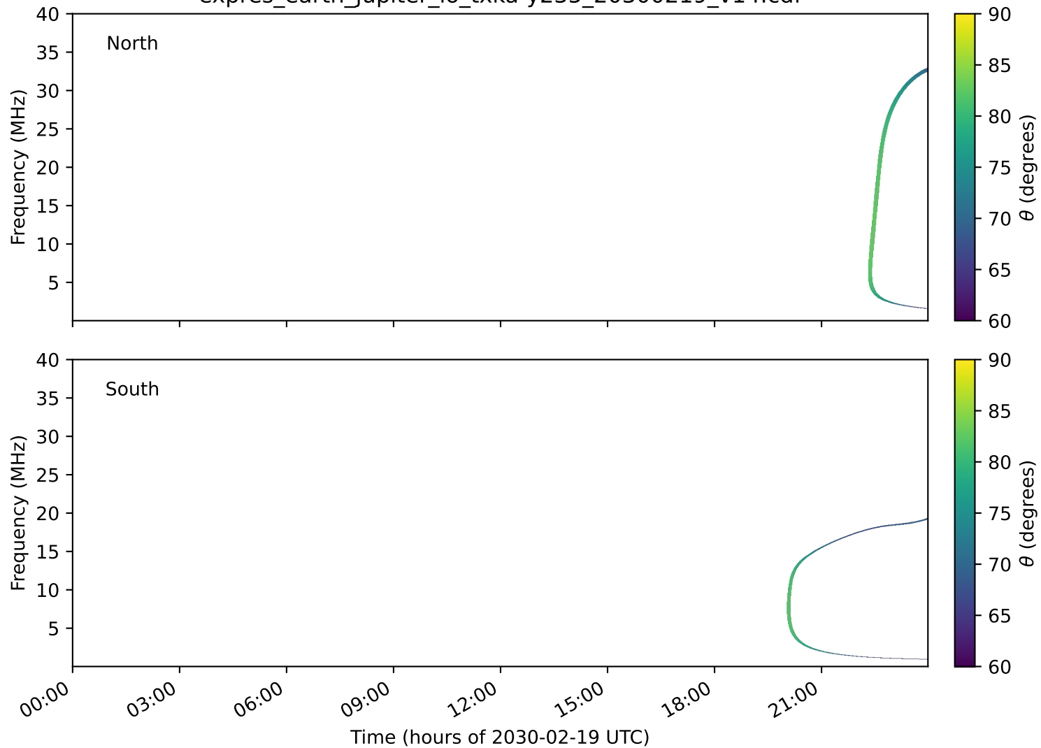
expres_earth_jupiter_io_txka-y235_20300219_v14.cdf
