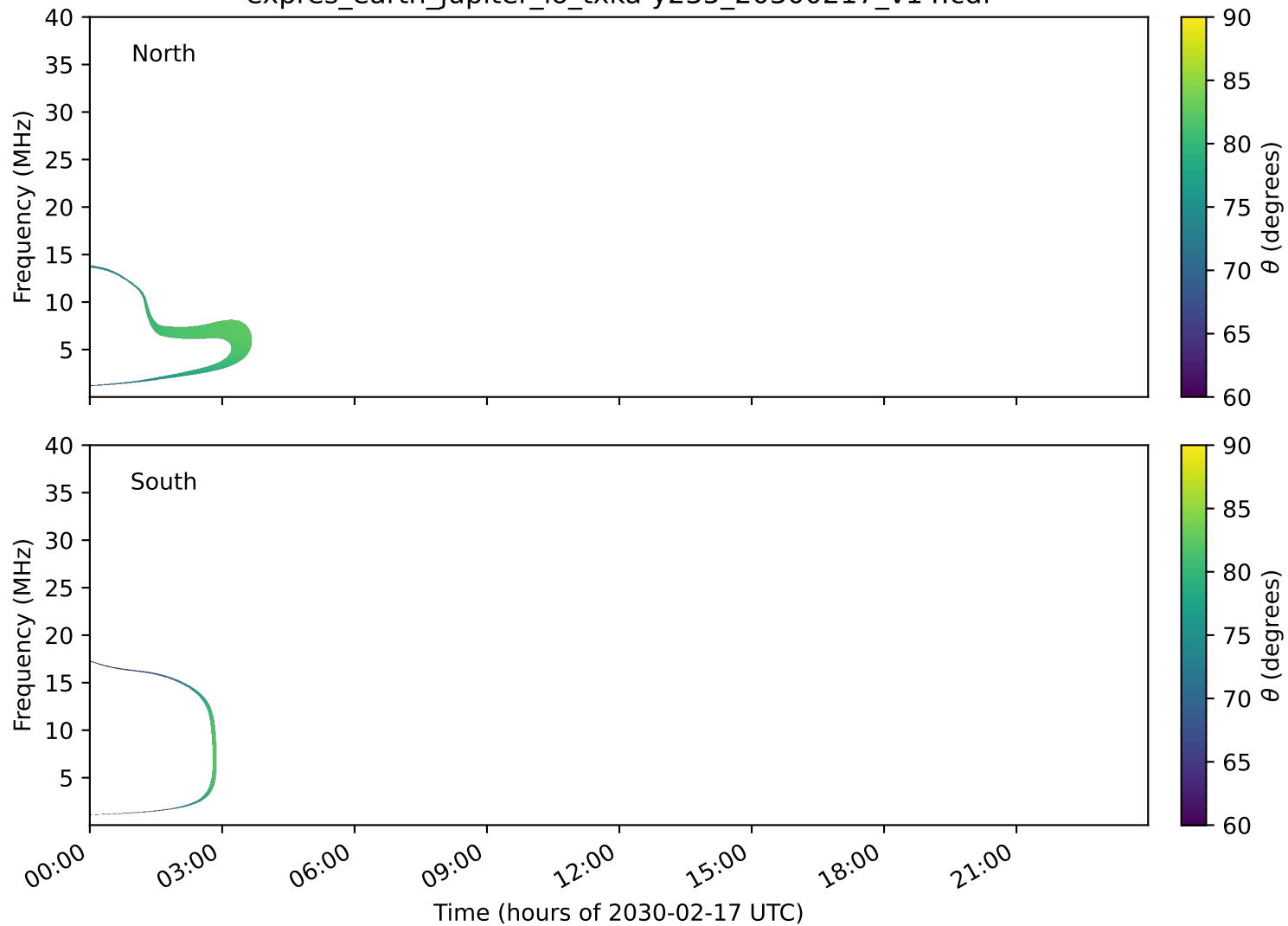
expres_earth_jupiter_io_txka-y235_20300217_v14.cdf
