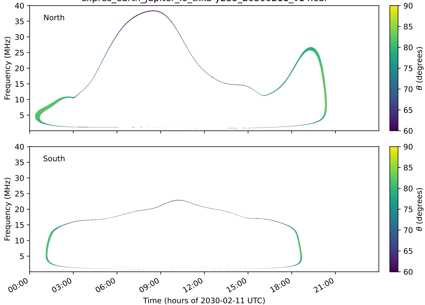
expres_earth_jupiter_io_txka-y235_20300211_v14.cdf
