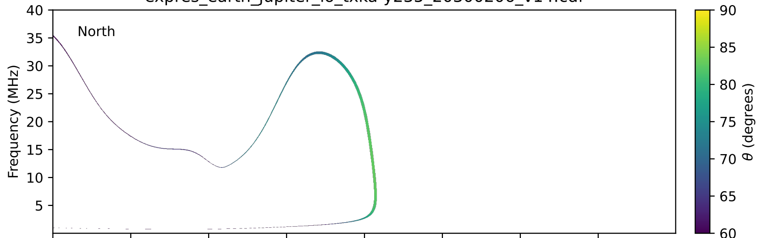
expres_earth_jupiter_io_txka-y235_20300206_v14.cdf
