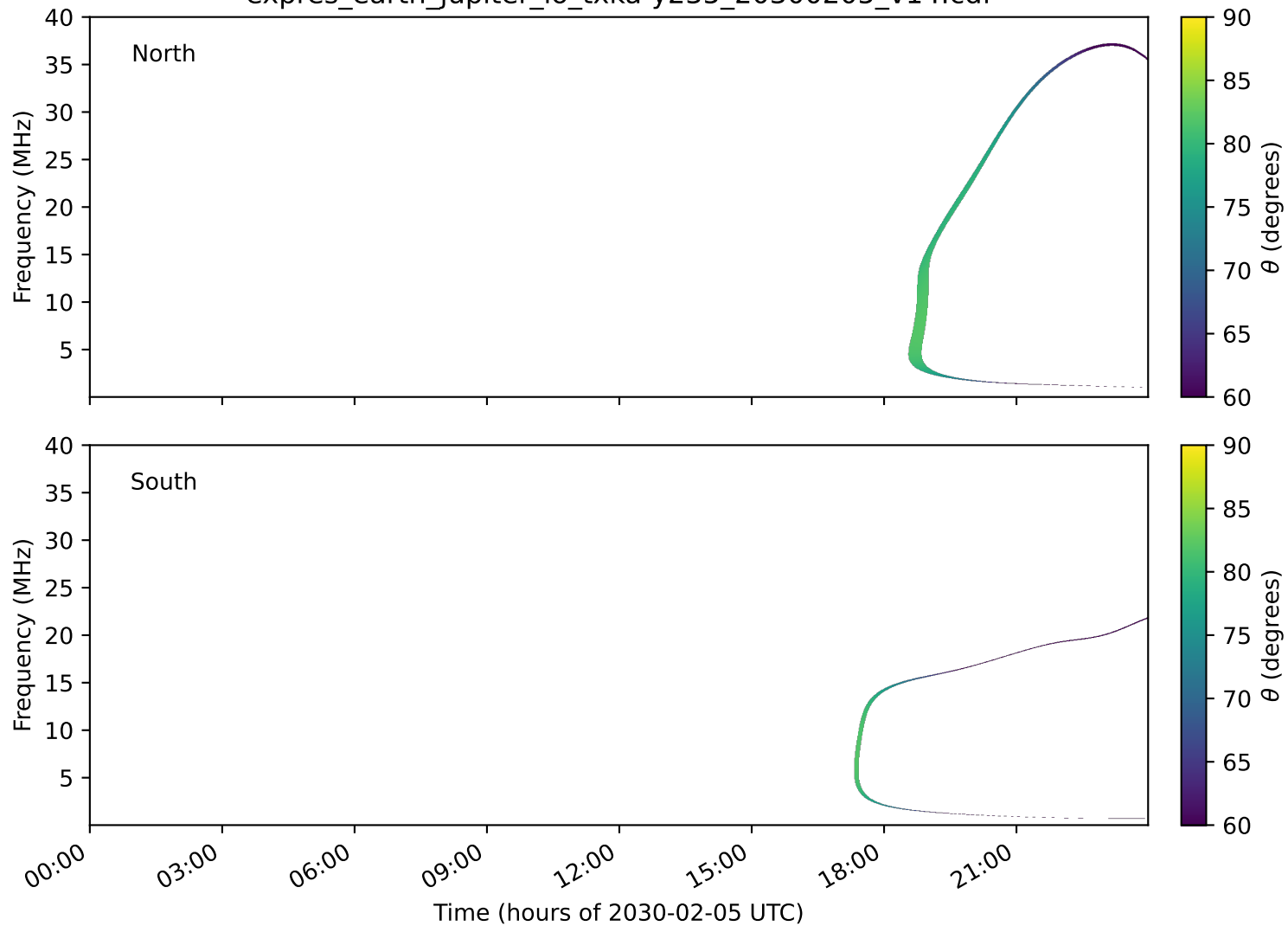
expres_earth_jupiter_io_txka-y235_20300205_v14.cdf
