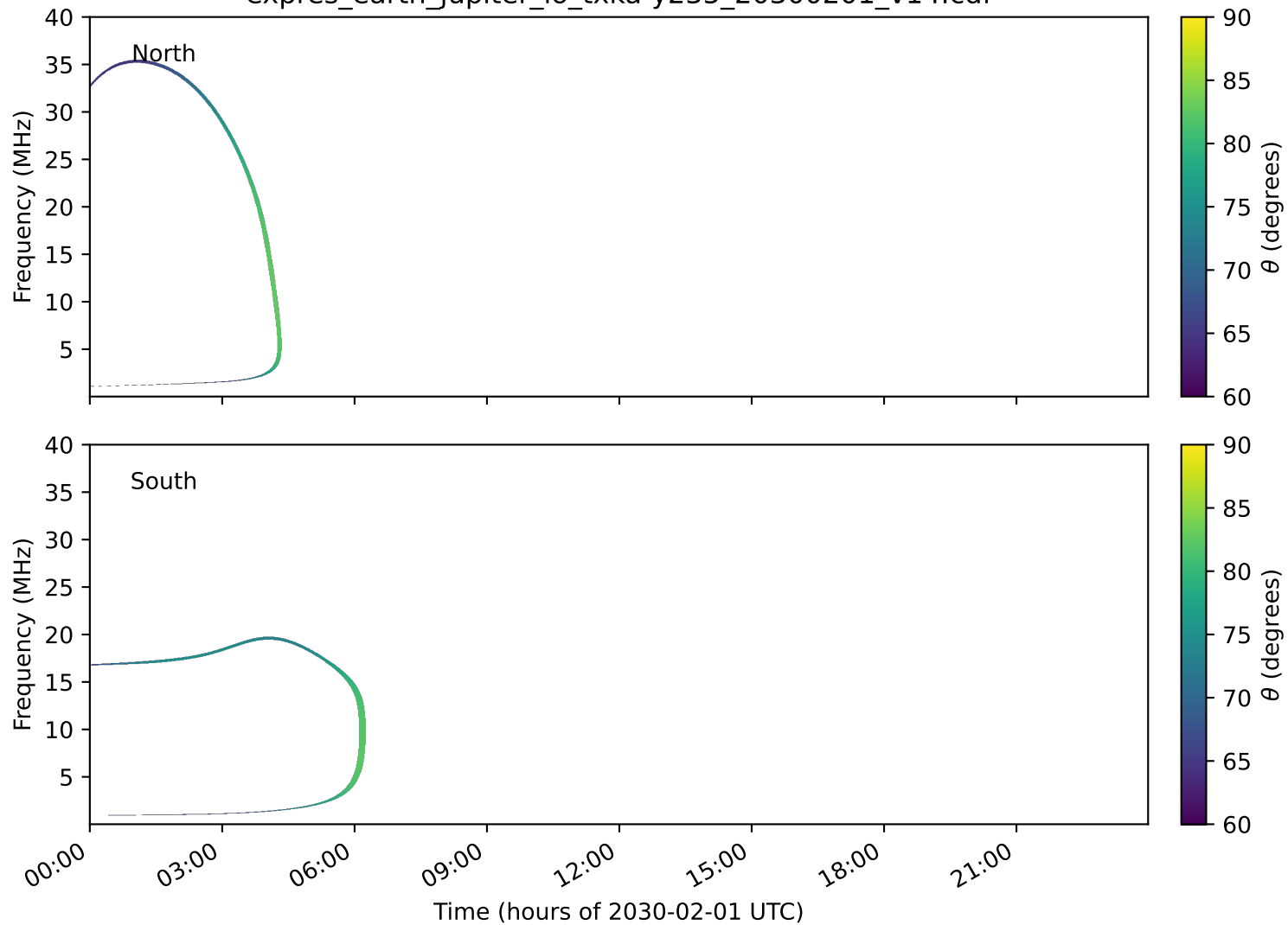
expres_earth_jupiter_io_txka-y235_20300201_v14.cdf
