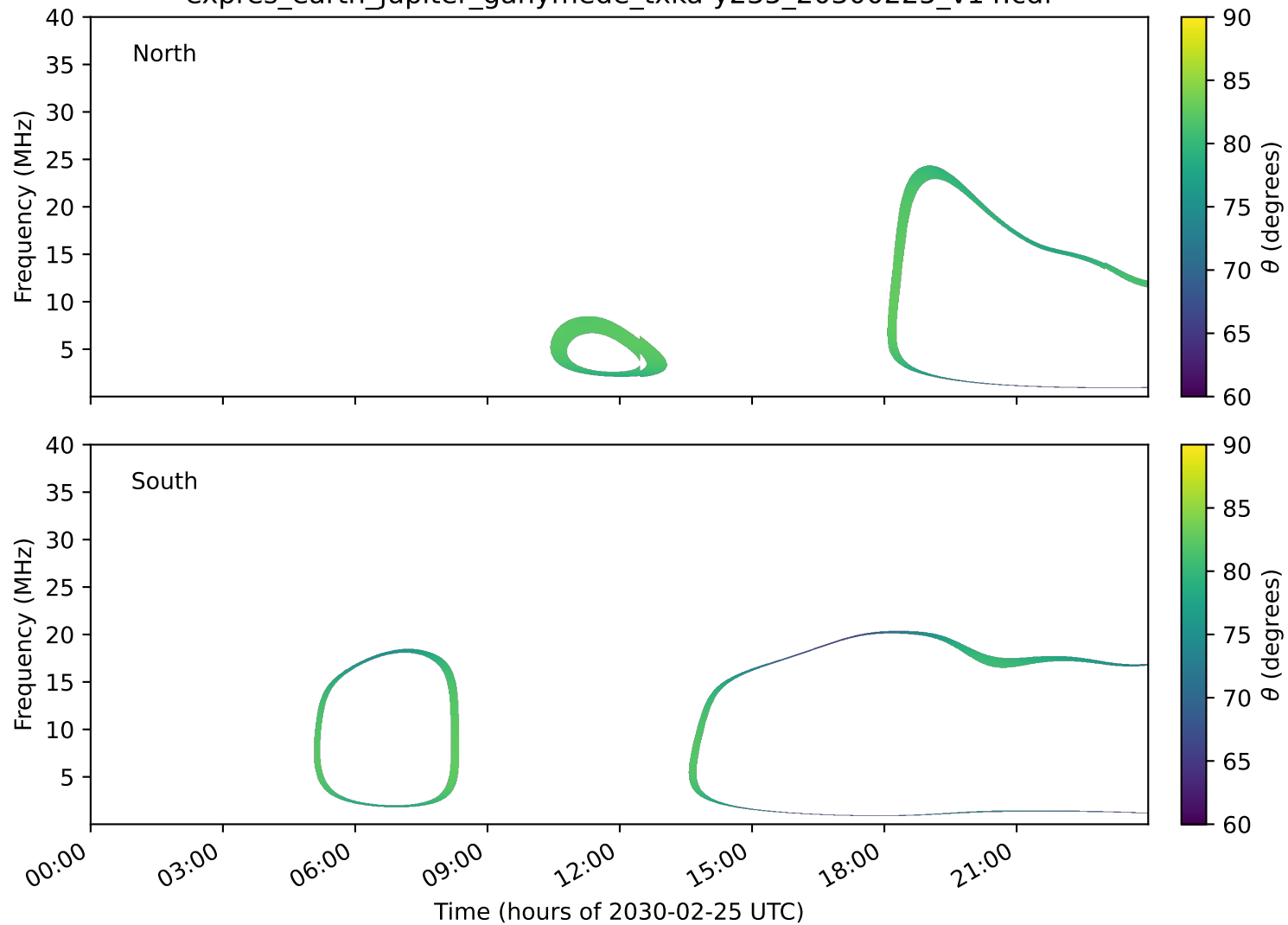
expres_earth_jupiter_ganymede_txka-y235_20300225_v14.cdf
