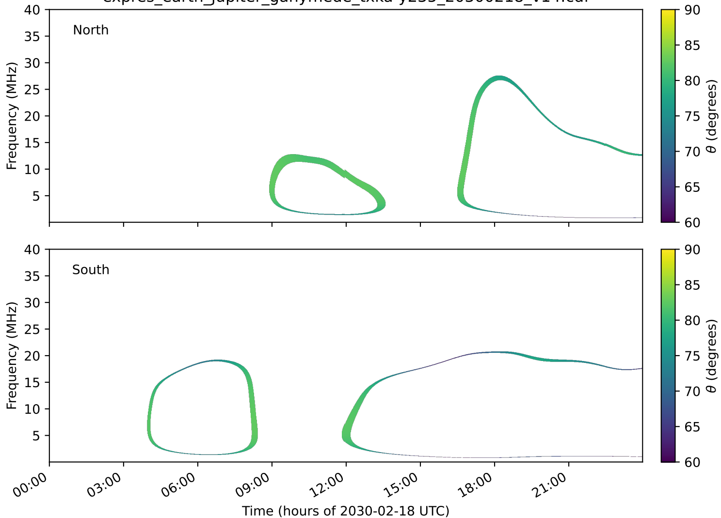
expres_earth_jupiter_ganymede_txka-y235_20300218_v14.cdf
