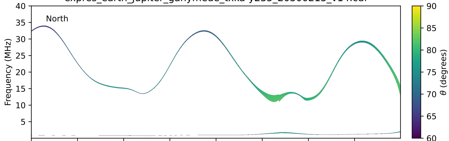
expres_earth_jupiter_ganymede_txka-y235_20300213_v14.cdf
