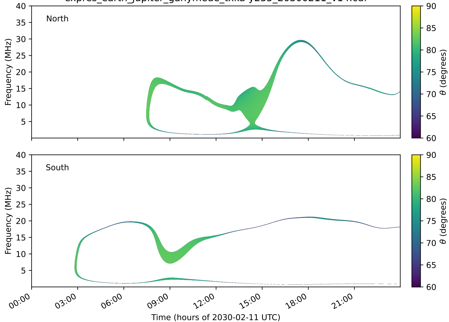
expres_earth_jupiter_ganymede_txka-y235_20300211_v14.cdf
