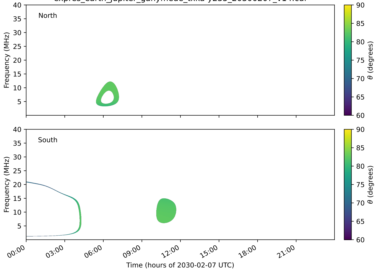
expres_earth_jupiter_ganymede_txka-y235_20300207_v14.cdf
