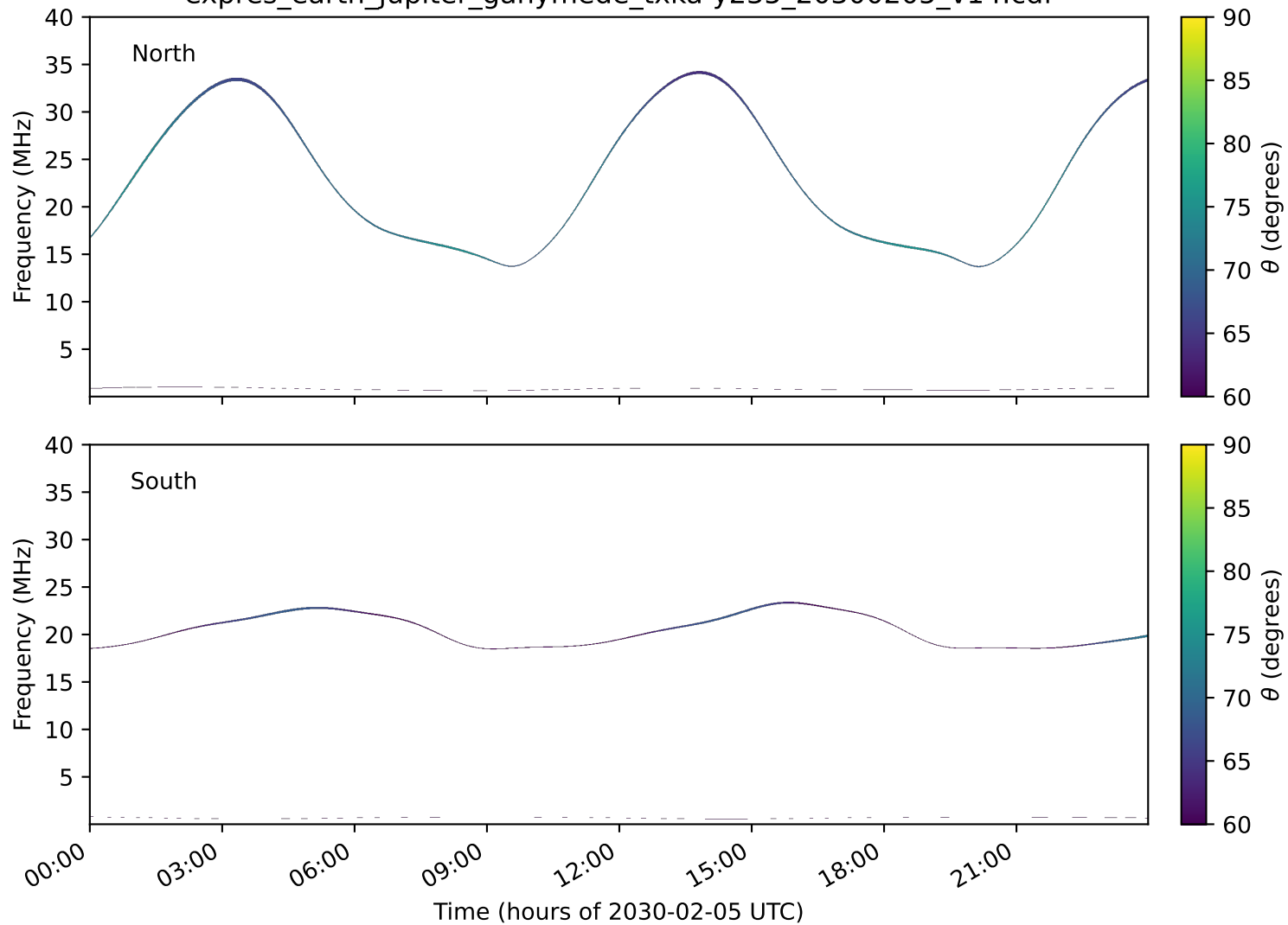
expres_earth_jupiter_ganymede_txka-y235_20300205_v14.cdf
