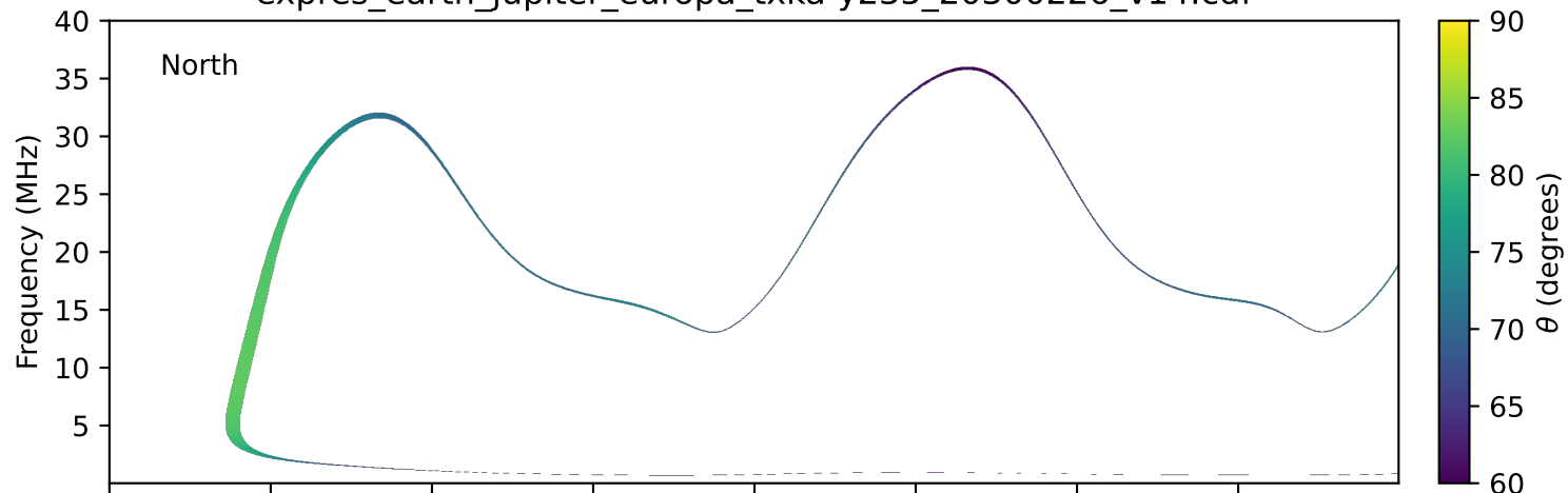
expres_earth_jupiter_europa_txka-y235_20300226_v14.cdf
