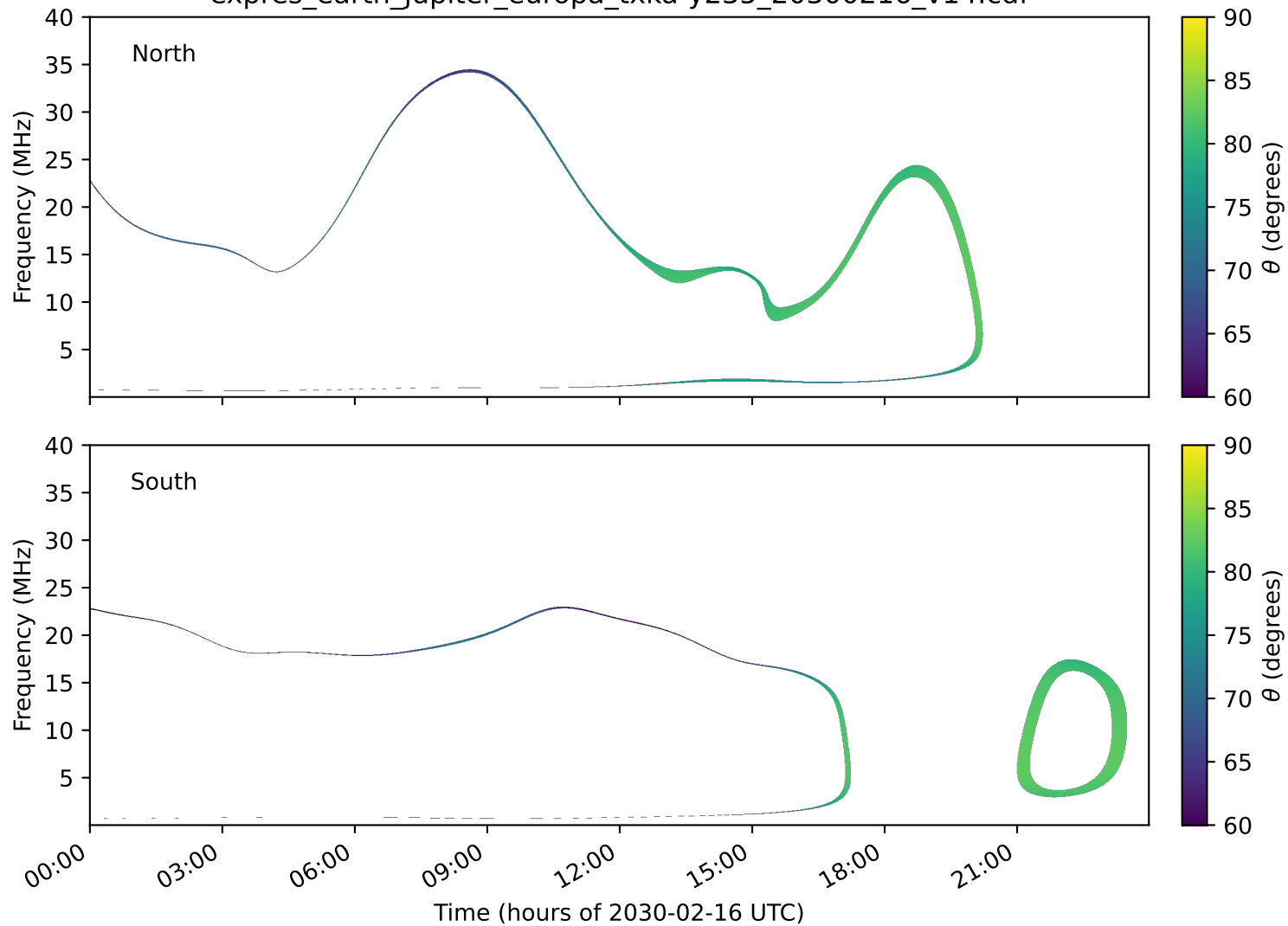
expres_earth_jupiter_europa_txka-y235_20300216_v14.cdf
