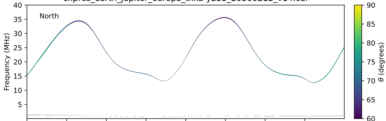
expres_earth_jupiter_europa_txka-y235_20300212_v14.cdf
