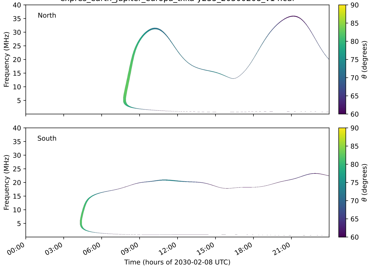
expres_earth_jupiter_europa_txka-y235_20300208_v14.cdf
