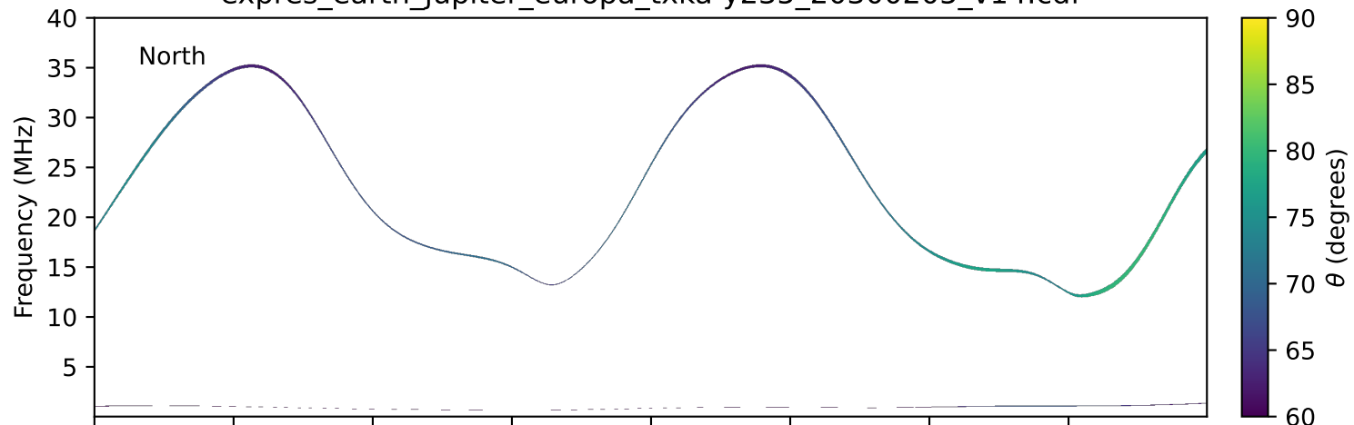
expres_earth_jupiter_europa_txka-y235_20300205_v14.cdf
