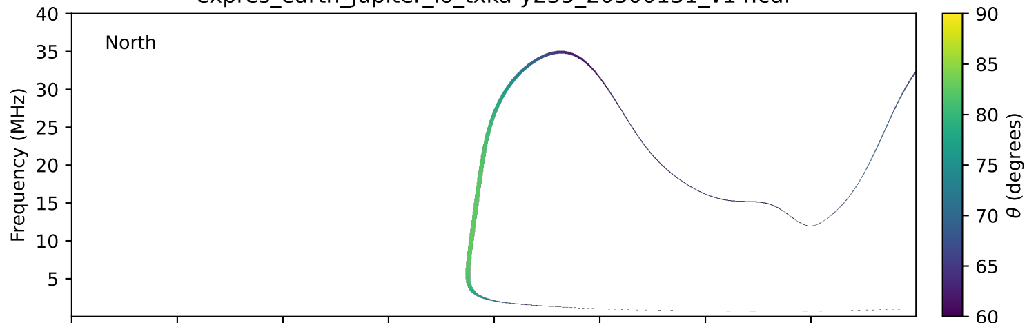
expres_earth_jupiter_io_txka-y235_20300131_v14.cdf
