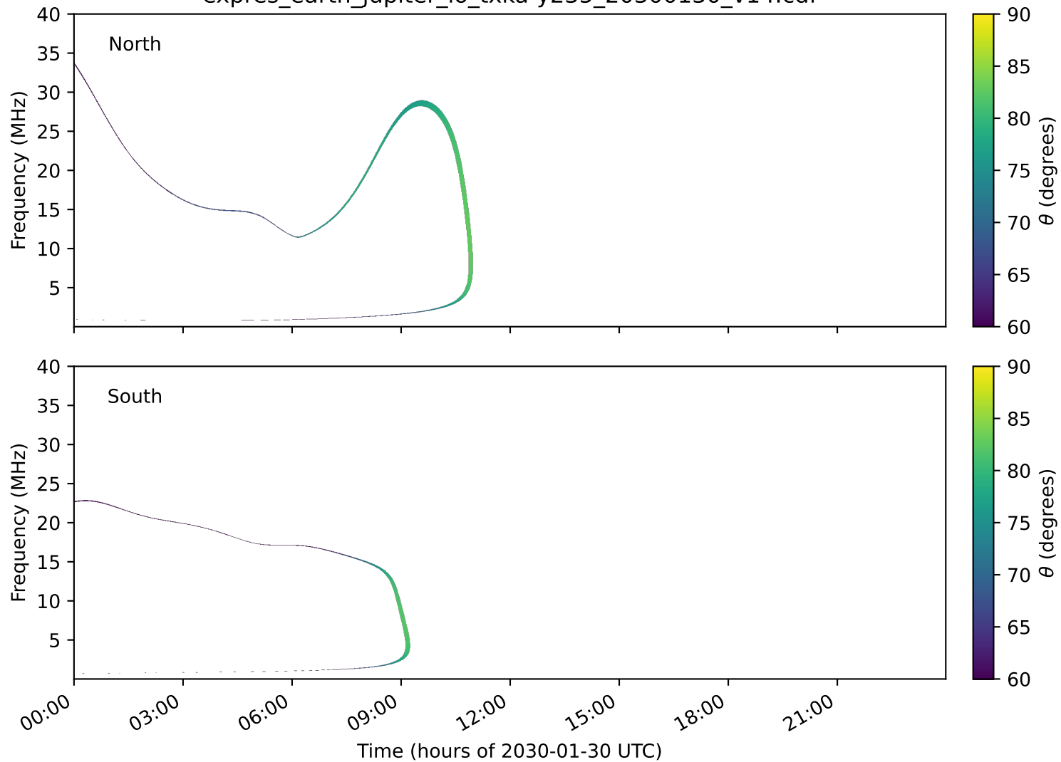
expres_earth_jupiter_io_txka-y235_20300130_v14.cdf
