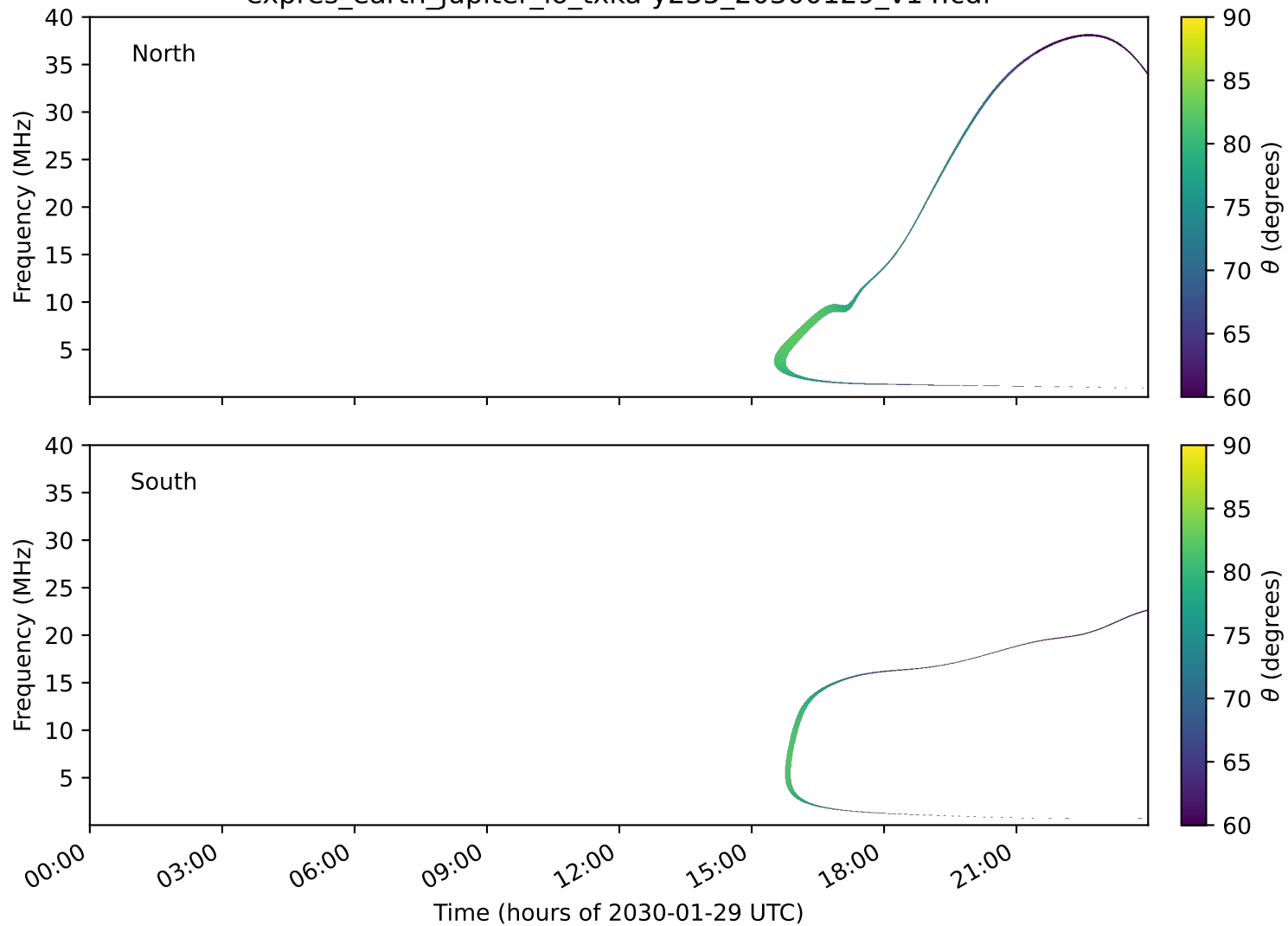
expres_earth_jupiter_io_txka-y235_20300129_v14.cdf
