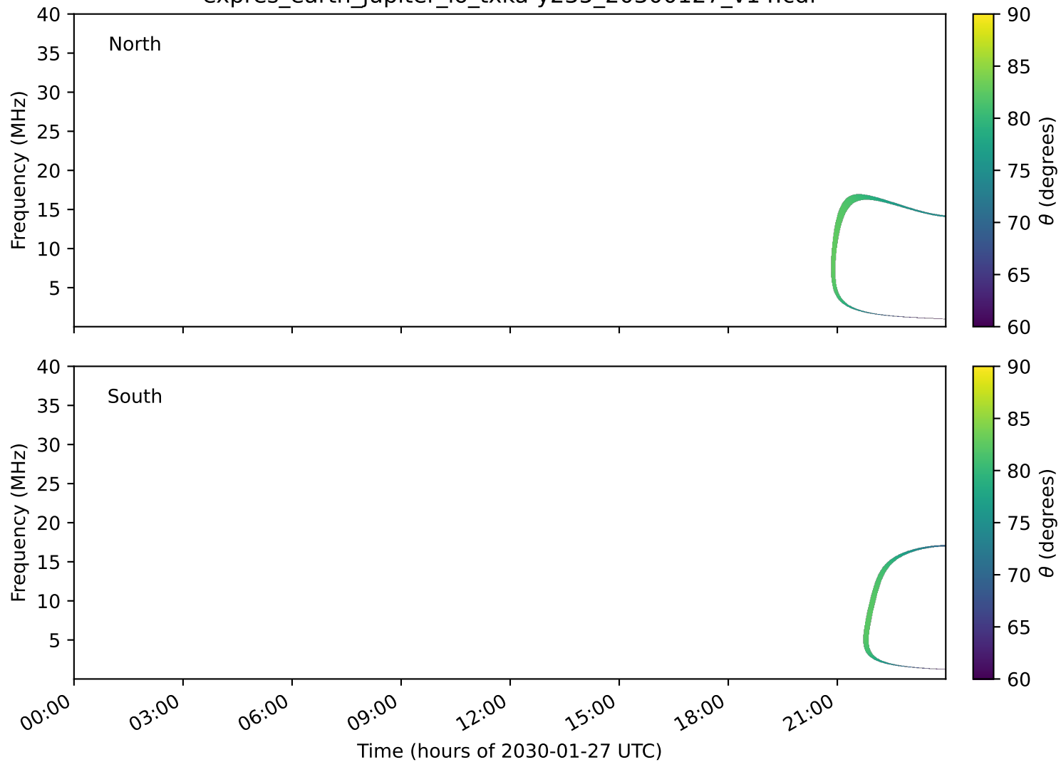
expres_earth_jupiter_io_txka-y235_20300127_v14.cdf
