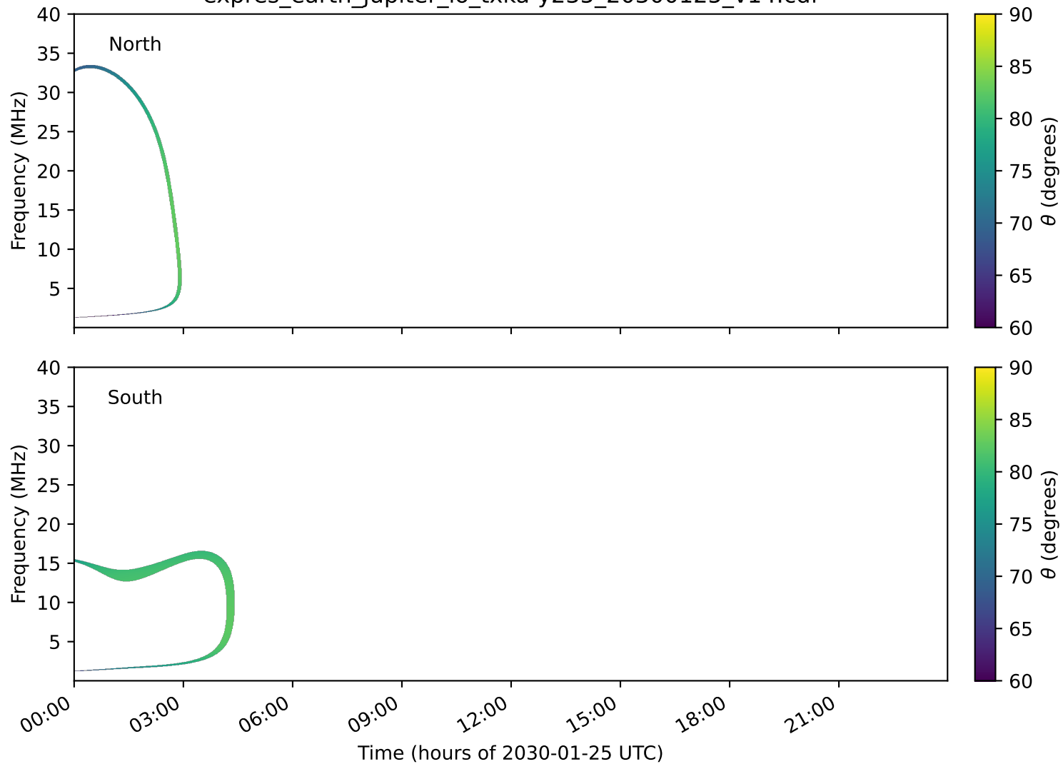
expres_earth_jupiter_io_txka-y235_20300125_v14.cdf
