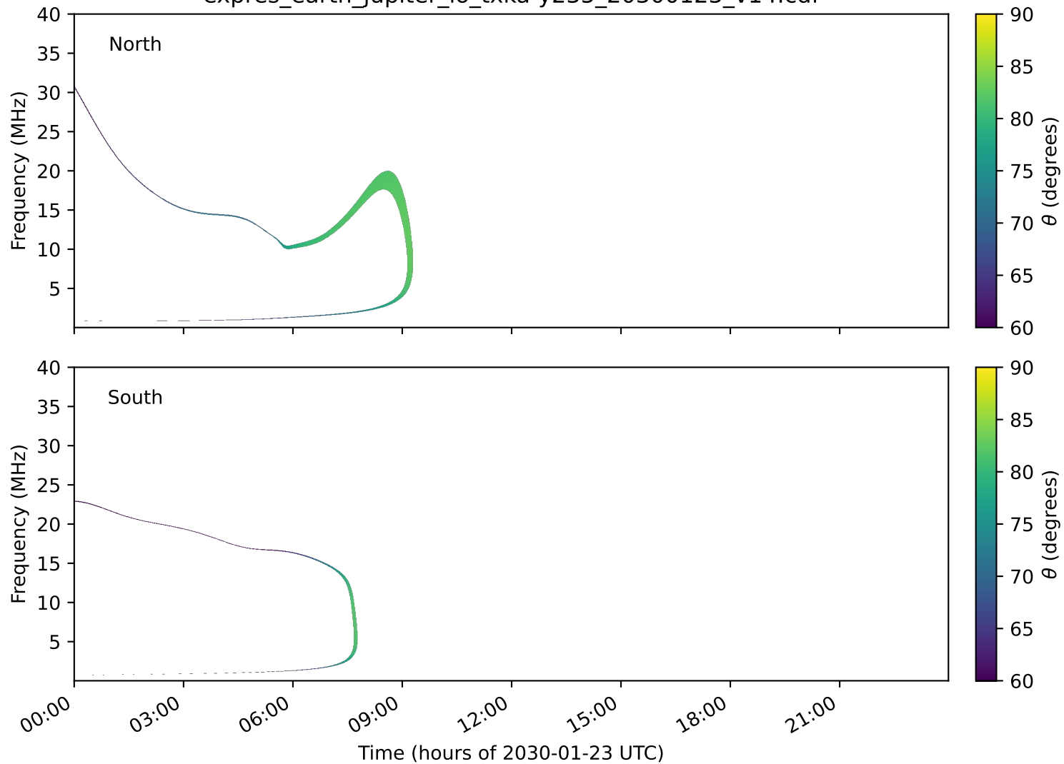
expres_earth_jupiter_io_txka-y235_20300123_v14.cdf
