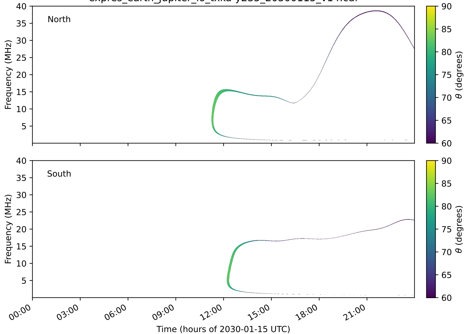
expres_earth_jupiter_io_txka-y235_20300115_v14.cdf
