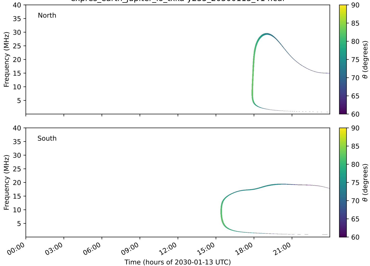
expres_earth_jupiter_io_txka-y235_20300113_v14.cdf
