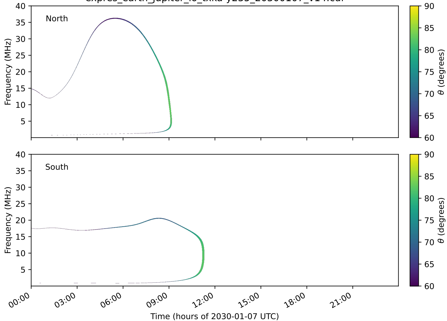
expres_earth_jupiter_io_txka-y235_20300107_v14.cdf
