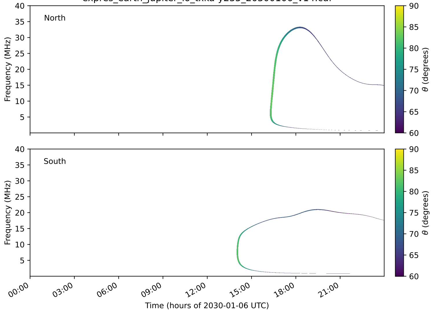
expres_earth_jupiter_io_txka-y235_20300106_v14.cdf
