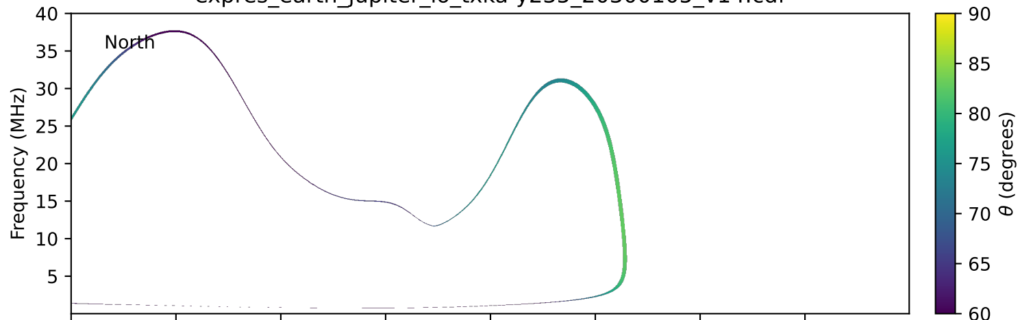
expres_earth_jupiter_io_txka-y235_20300105_v14.cdf
