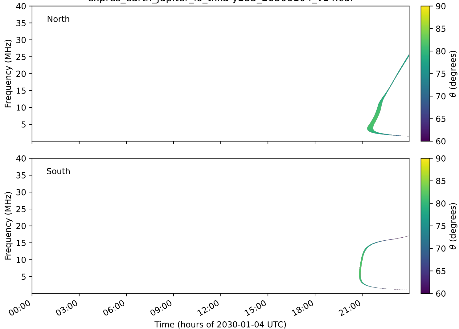
expres_earth_jupiter_io_txka-y235_20300104_v14.cdf
