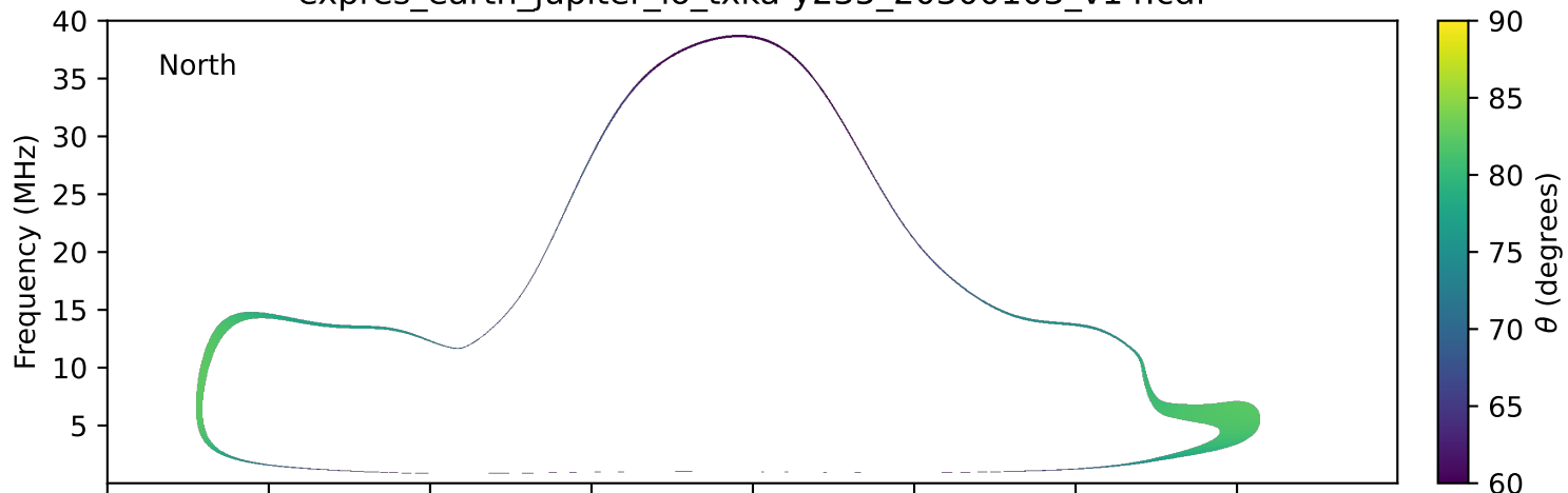
expres_earth_jupiter_io_txka-y235_20300103_v14.cdf
