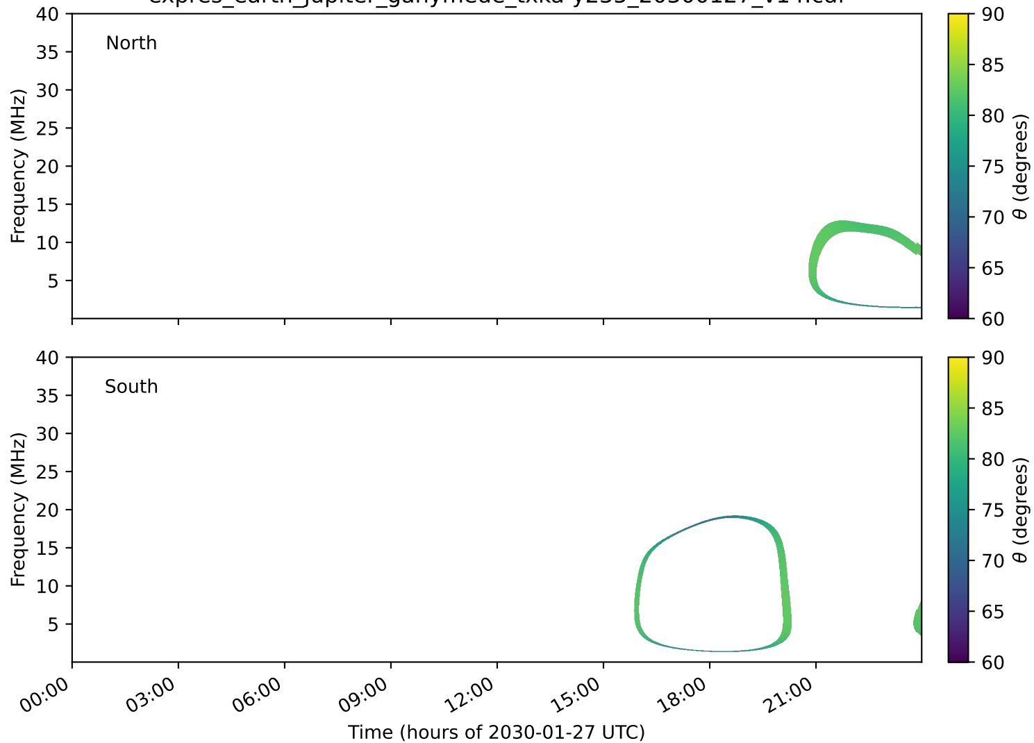
expres_earth_jupiter_ganymede_txka-y235_20300127_v14.cdf
