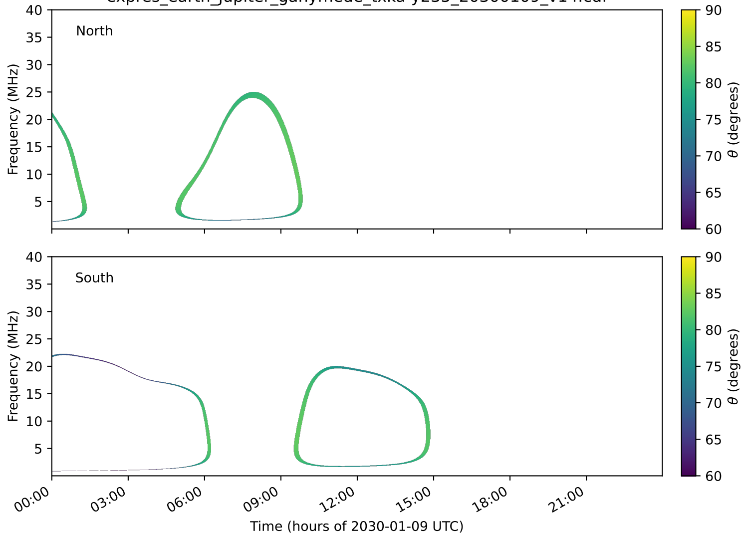
expres_earth_jupiter_ganymede_txka-y235_20300109_v14.cdf
