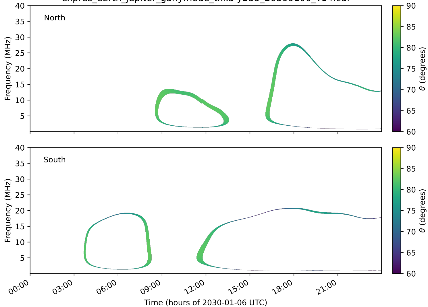
expres_earth_jupiter_ganymede_txka-y235_20300106_v14.cdf
