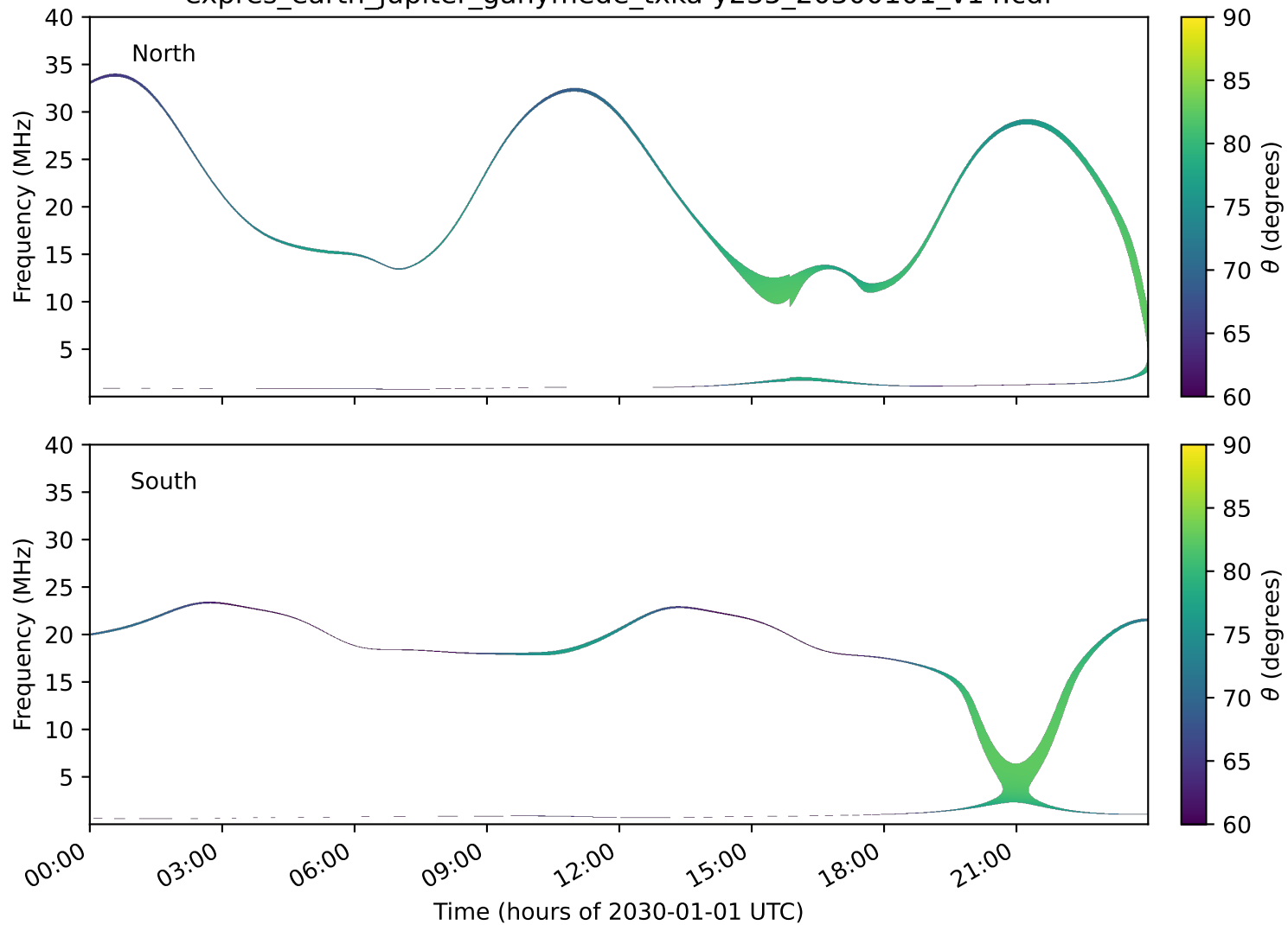
expres_earth_jupiter_ganymede_txka-y235_20300101_v14.cdf
