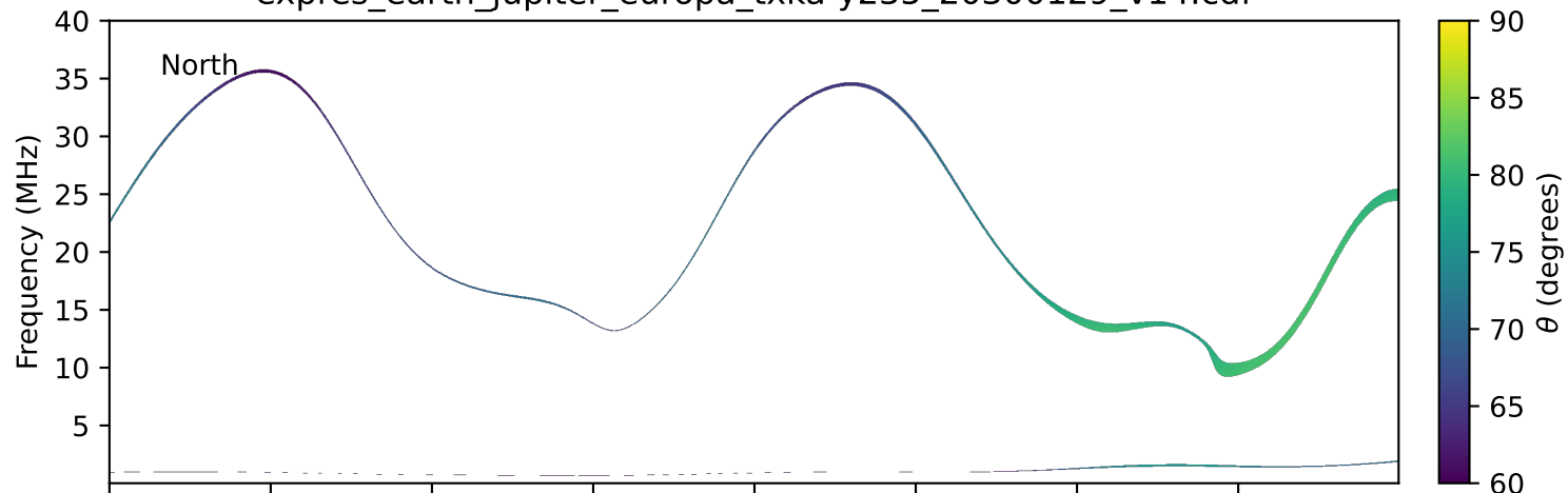
expres_earth_jupiter_europa_txka-y235_20300129_v14.cdf
