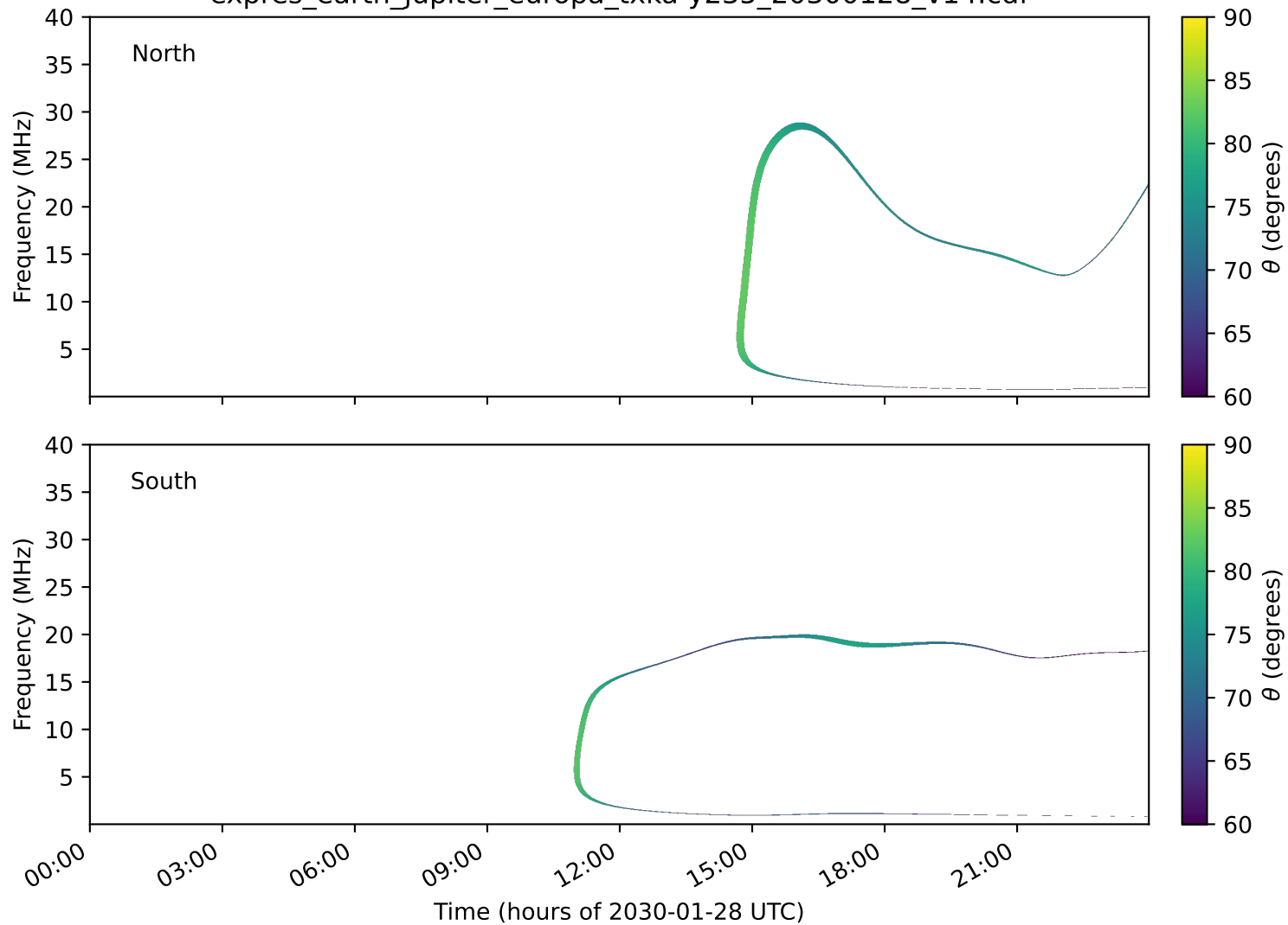
expres_earth_jupiter_europa_txka-y235_20300128_v14.cdf
