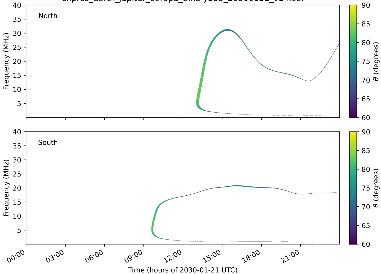
expres_earth_jupiter_europa_txka-y235_20300121_v14.cdf
