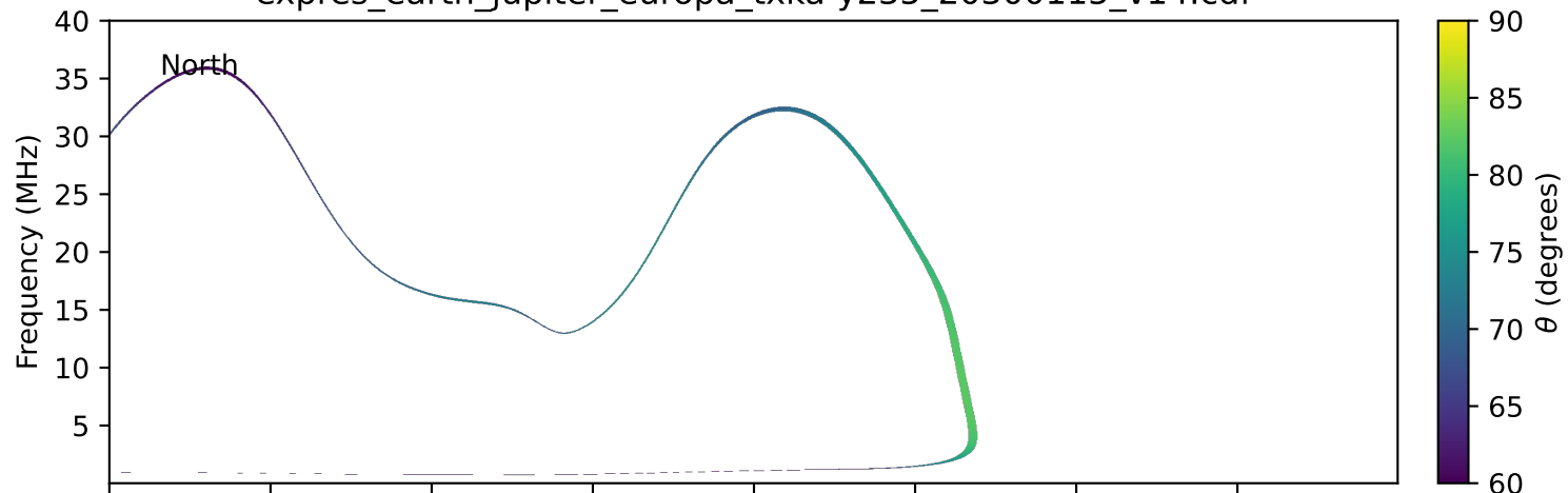
expres_earth_jupiter_europa_txka-y235_20300115_v14.cdf
