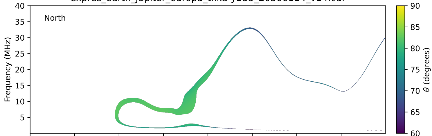
expres_earth_jupiter_europa_txka-y235_20300114_v14.cdf
