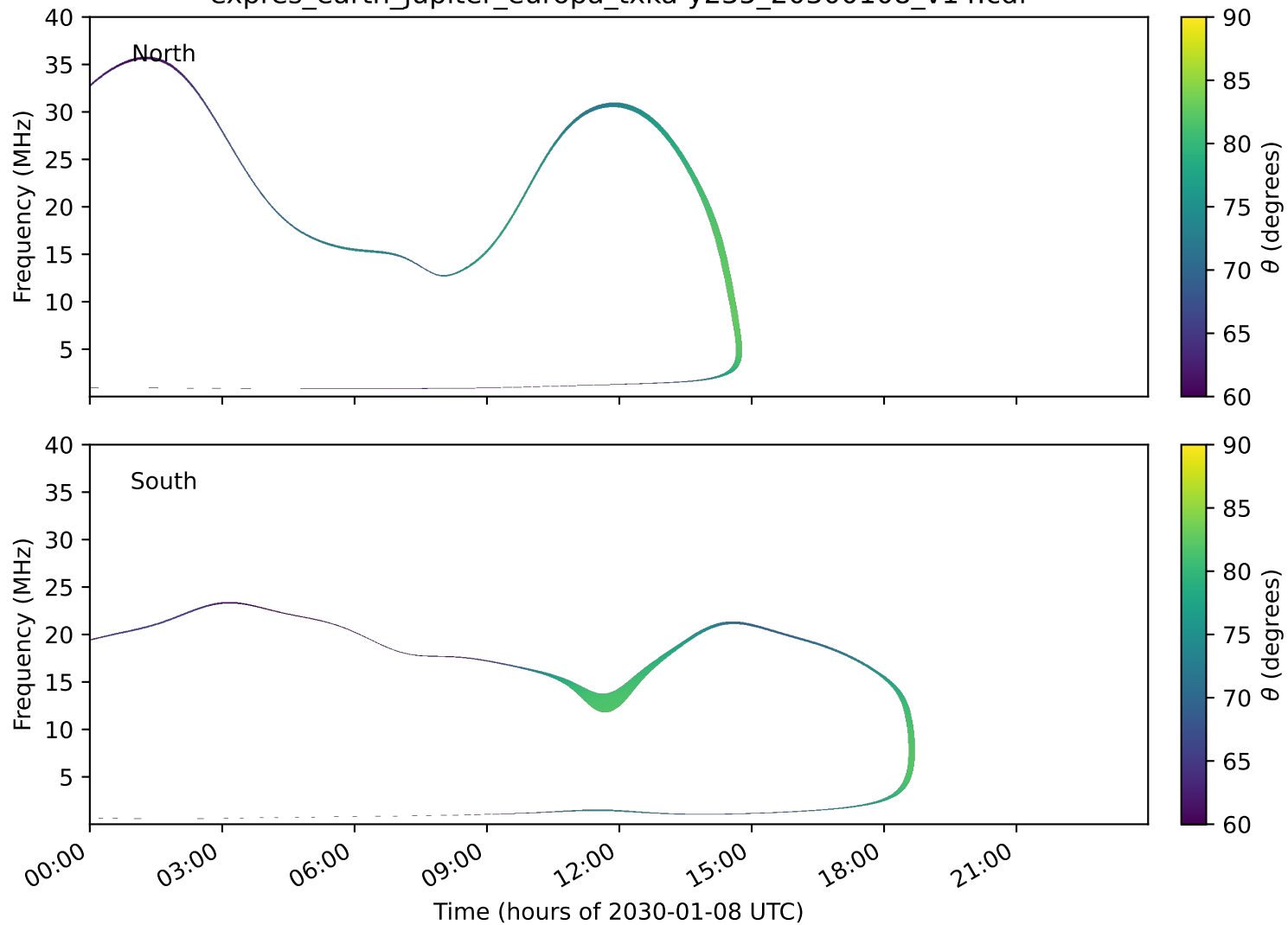
expres_earth_jupiter_europa_txka-y235_20300108_v14.cdf
