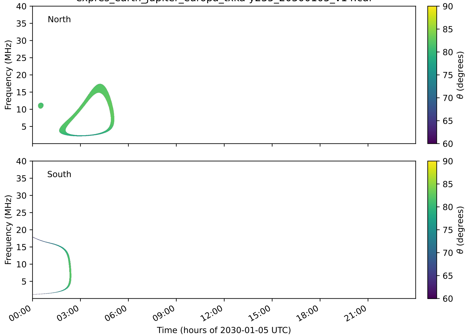
expres_earth_jupiter_europa_txka-y235_20300105_v14.cdf
