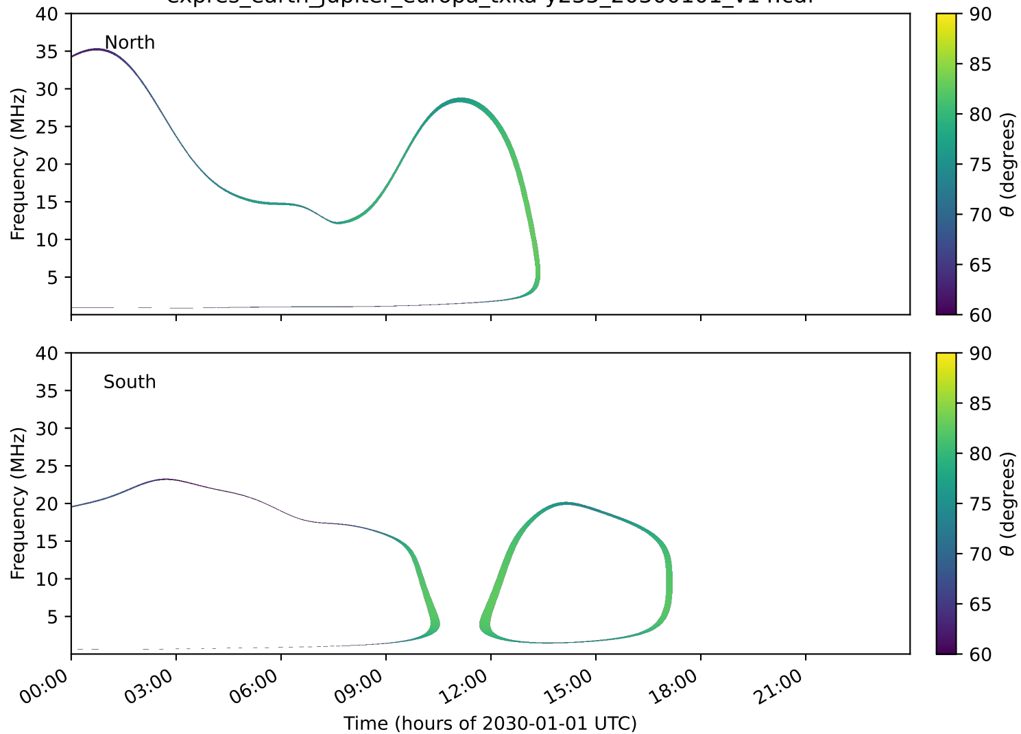
expres_earth_jupiter_europa_txka-y235_20300101_v14.cdf
