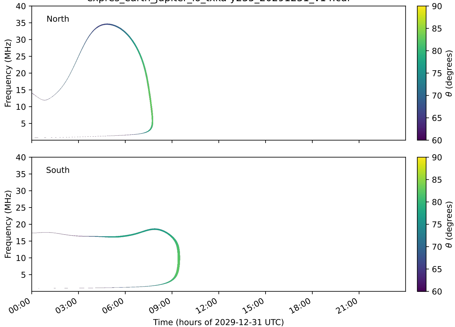
expres_earth_jupiter_io_txka-y235_20291231_v14.cdf
