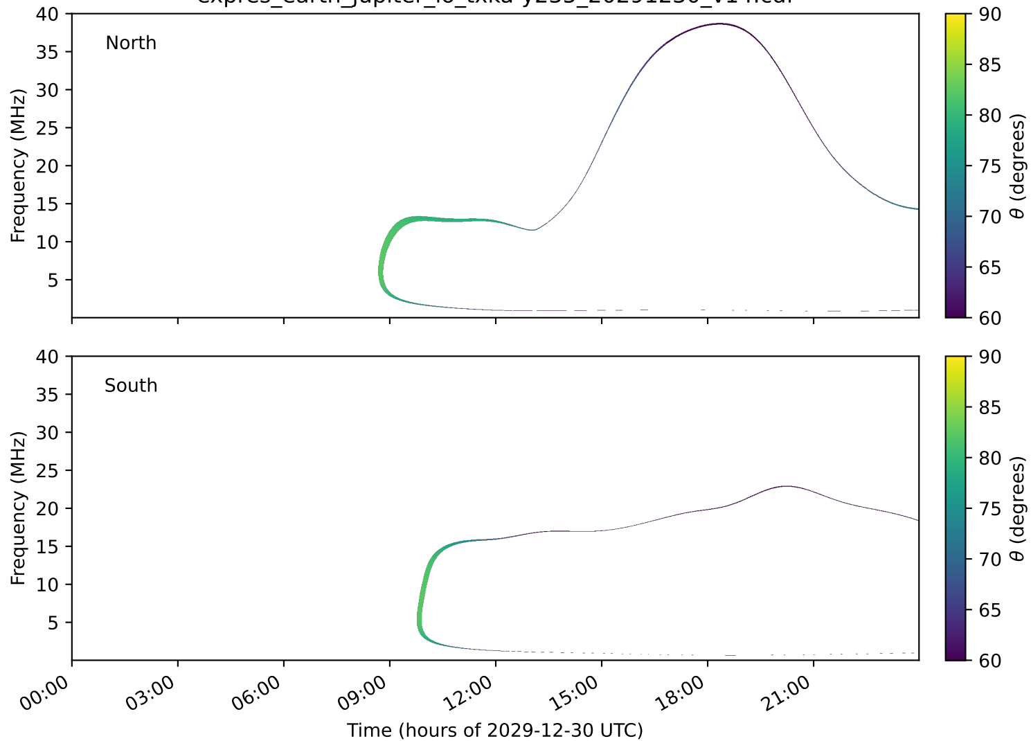
expres_earth_jupiter_io_txka-y235_20291230_v14.cdf
