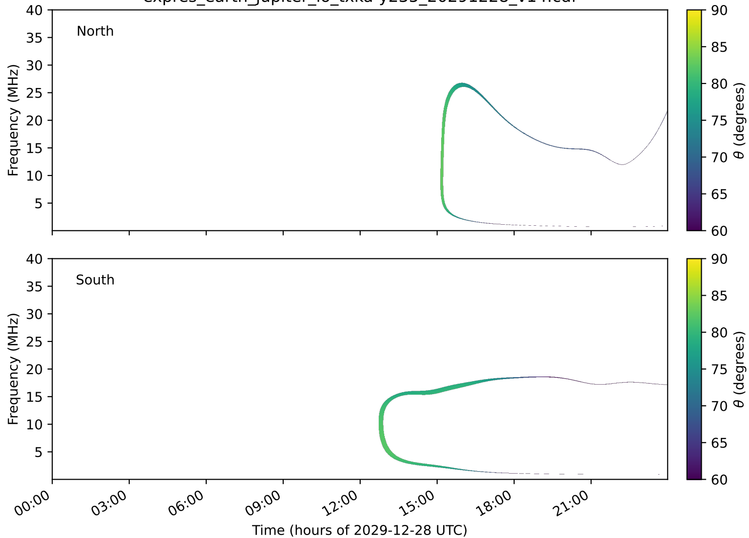
expres_earth_jupiter_io_txka-y235_20291228_v14.cdf
