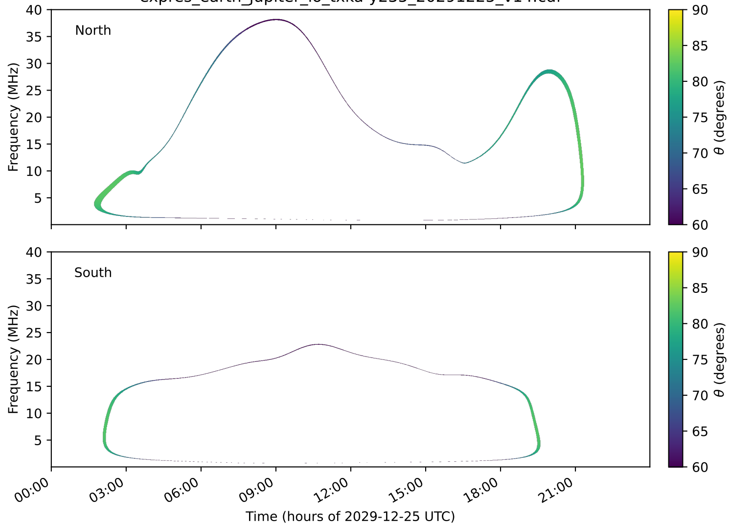
expres_earth_jupiter_io_txka-y235_20291225_v14.cdf
