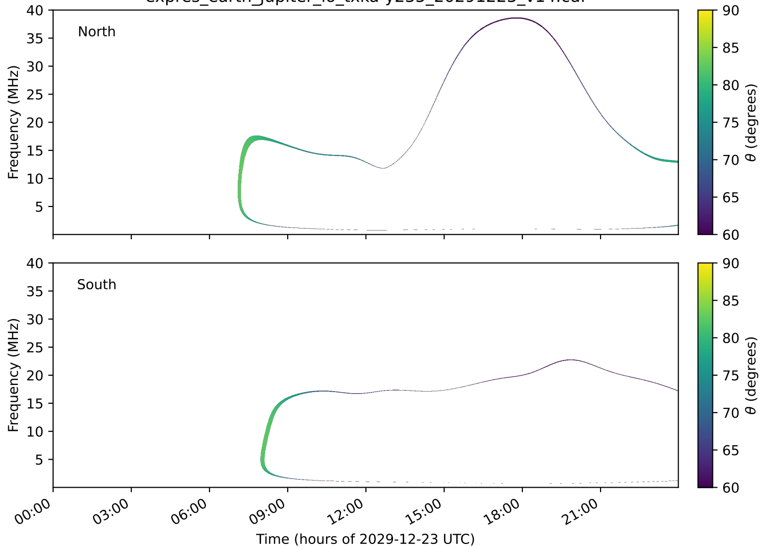
expres_earth_jupiter_io_txka-y235_20291223_v14.cdf
