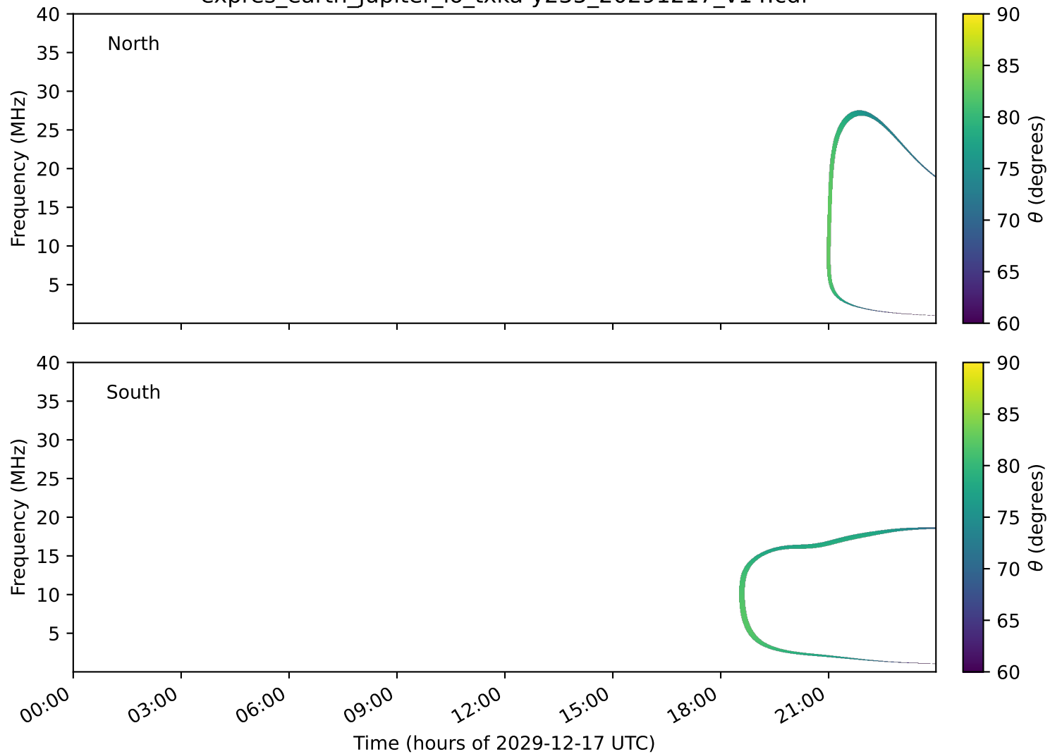
expres_earth_jupiter_io_txka-y235_20291217_v14.cdf
