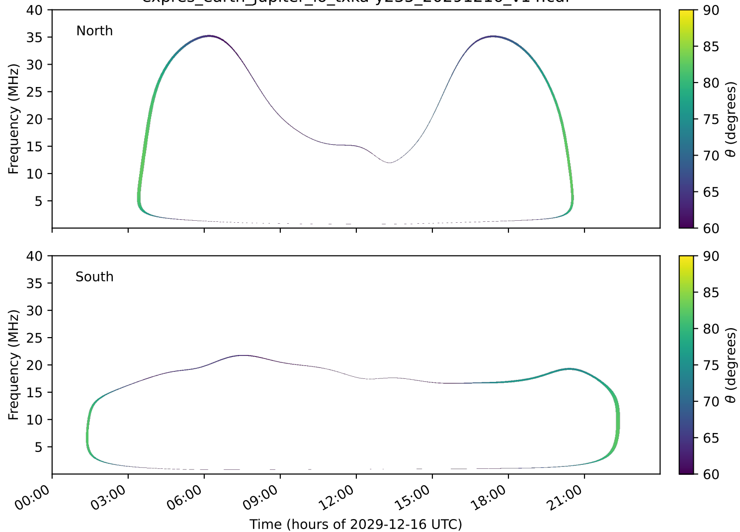
expres_earth_jupiter_io_txka-y235_20291216_v14.cdf
