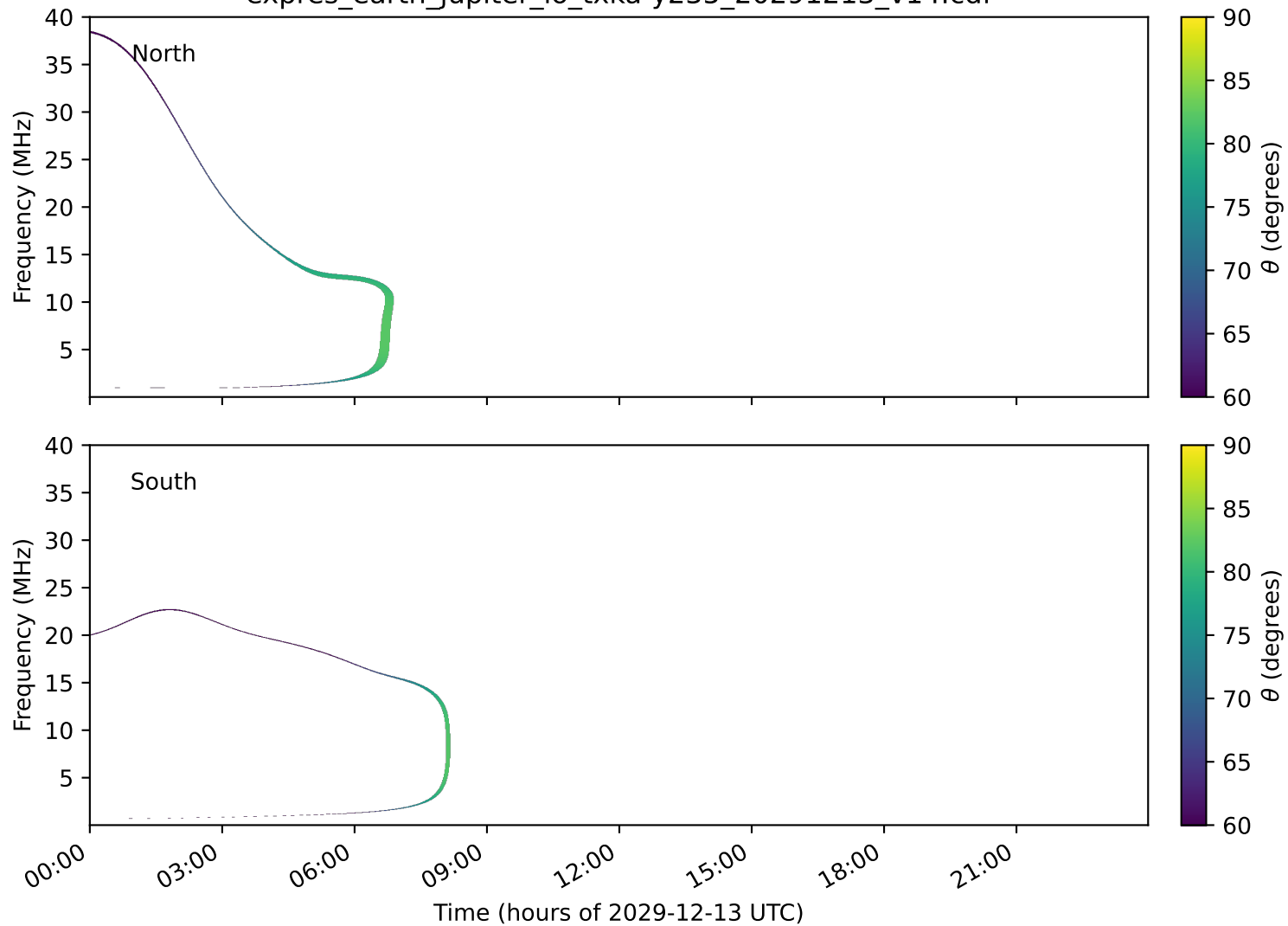
expres_earth_jupiter_io_txka-y235_20291213_v14.cdf
